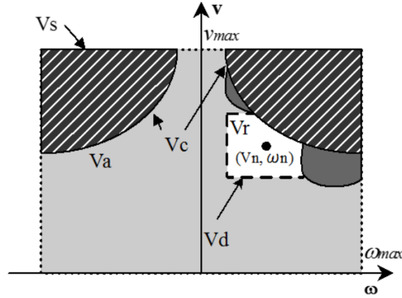
Fig. 4. Velocity space
